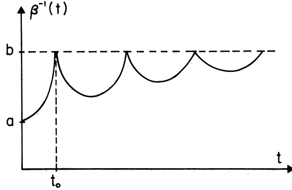
FIG. 1. Time dependence of \beta^{-1}(t) . The initial and final values of \beta^{-1} are: a = 2\langle H \rangle / 3N - p_0^2 / 3m , b = 2\langle H \rangle / 3N .
